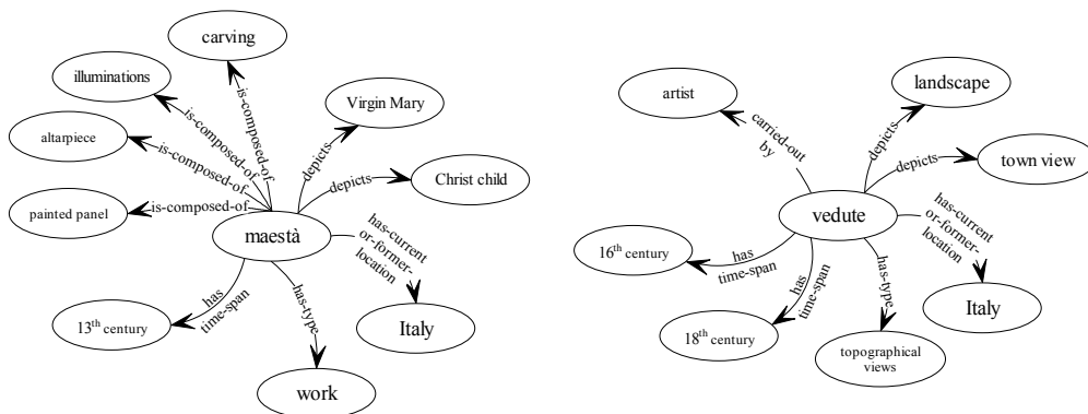
Figure 3. Extracted conceptualisation (in graphical form) of the terms maesta #1 and vedute #1 (sense numbers are omitted for clarity).
