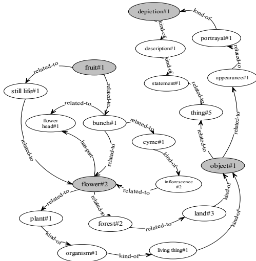
Figure 2. Semantic Interconnections selected by the SSI algorithm when given the word list: “depiction, fruit, flower, object”.
