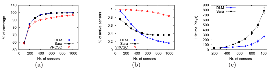
Fig. 10. Adjustable sensors, heterogeneous setting. Percentage of the AoI covered (a), percentage of awake sensors (b) and network lifetime (c). The network lifetime is defined as the time at which coverage falls below 80%.
