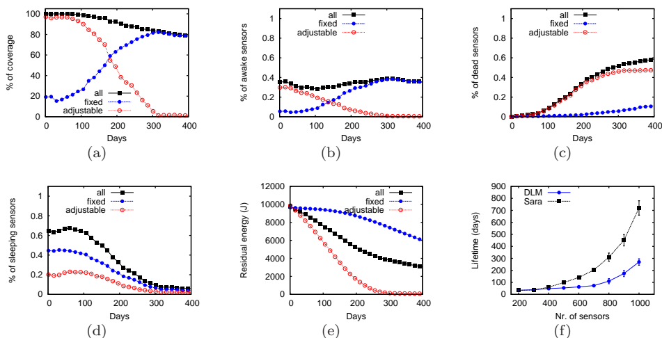
Fig. 13. Mixed sensors: scenario B. The maximum radius of the adjustable sensors is 6m while the radius of fixed sensors is 3m. Case of 900 sensors: 50% fixed and 50% adjustable. Coverage of the AoI (a), awake sensors (b), dead sensors (c), sleeping sensors (d) and residual energy (e). Lifetime of the network when varying the number of sensors (50 % fixed, 50% adjustable sensors).
