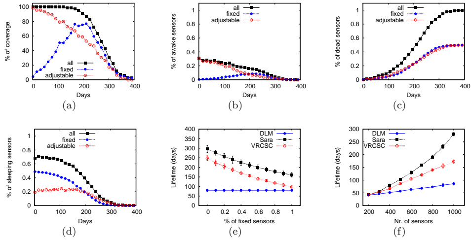
Fig. 12. Mixed sensors: Scenario A. The maximum radius of adjustable sensors and the radius of fixed sensors are 6m. Case of 900 sensors: 50 % fixed and 50 % adjustable range. Coverage of the AoI (a), awake sensors (b), dead sensors (c), and sleeping sensors (d). Lifetime of the network by varying the percentage of fixed sensors with respect to total (e). Lifetime of the network by varying the number of available sensors (50 % of each class) (f).
