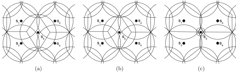
Fig. 7. About Pareto optimality. Initial configuration (a). Selective activation with VRCSC (b) and SARA (c).
