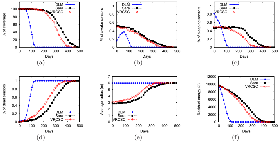
Fig. 8. Adjustable sensors: homogeneous setting. Comparative analysis of SARA, DLM and VRCSC. Percentage of AoI covered (a), percentage of awake sensors (b), percentage of sleeping sensors (c), percentage of dead sensors (d). Average radius of the awake sensors (e) and average residual energy per sensor (f). Scenario with 900 sensors.
