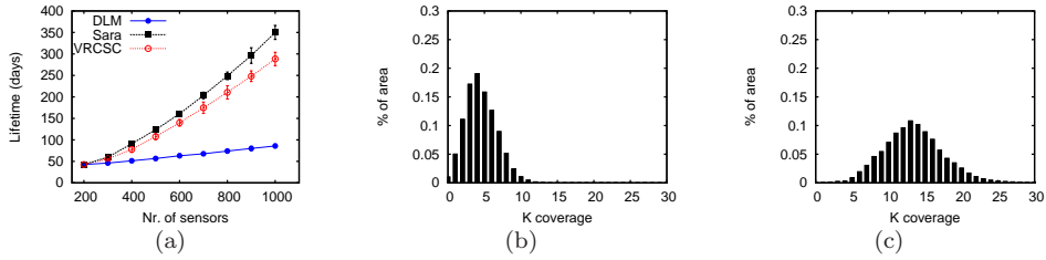
Fig. 9. Adjustable sensors, homogeneous setting. Lifetime (a) and percentage of the AoI which is covered by K sensors, for different values of K , when 300 sensors (b) and 900 sensors (c) are deployed over the AoI.
