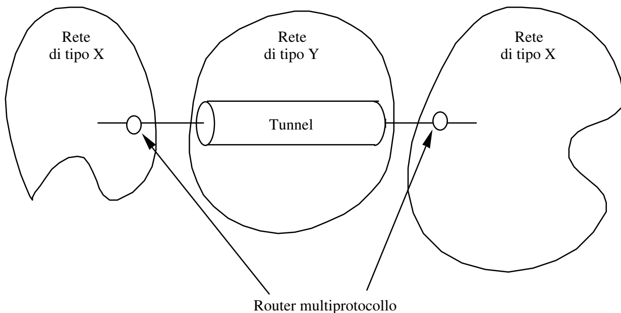
Figura 5-6: Tunneling
