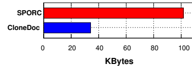
Figure 3: Cellular network traffic with SPORC and CloneDoc.
